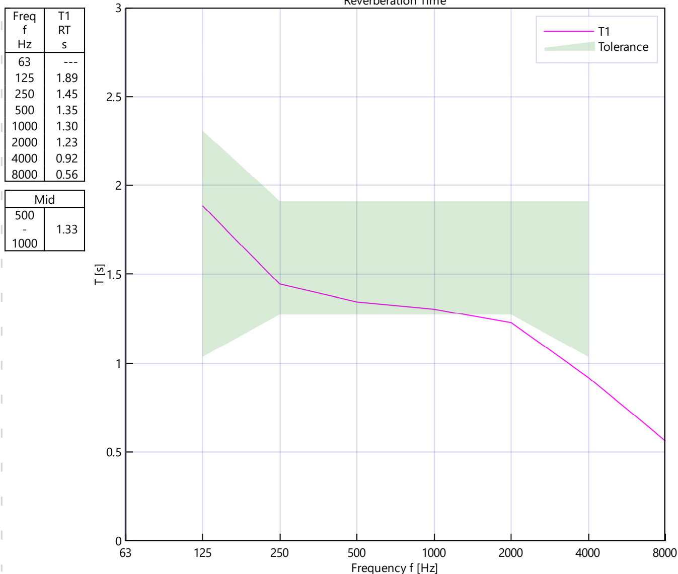
Reverberation Time
