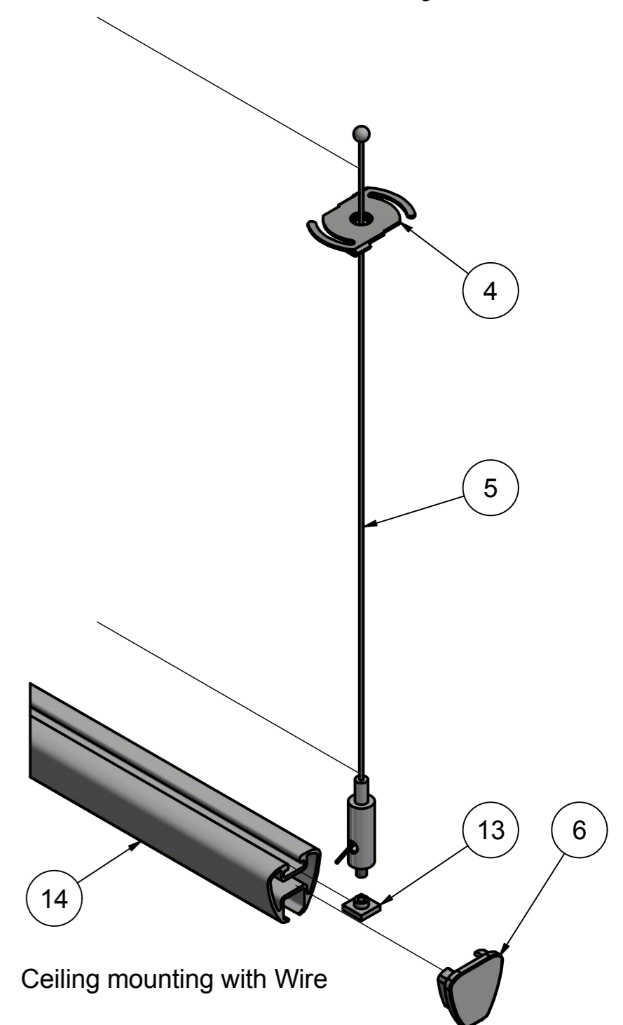
Roof mounting with Wire
